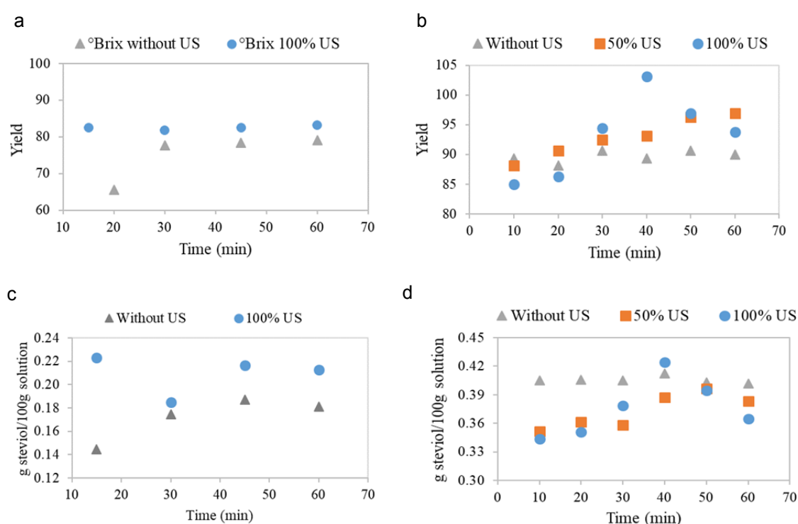
Figure 4: Yield calculated at the outlet cell with a leaves concentration of 50 g/L (a) °Bx concentration with D[3,2] of 17 \mu\text{m} (set 3) (b) °Bx concentration for D[3,2] of 18 \mu\text{m} (leaves and branches, set 2) (c) steviol concentration measured by HPLC (set 3), (d) steviol concentration measured by HPLC (set 2).
